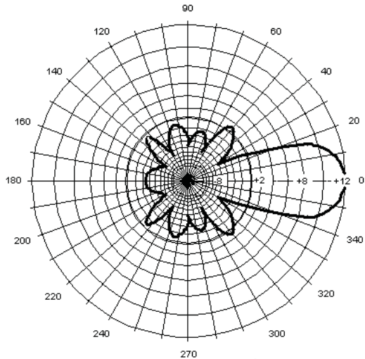
MYA45012 Horizontal Pattern
