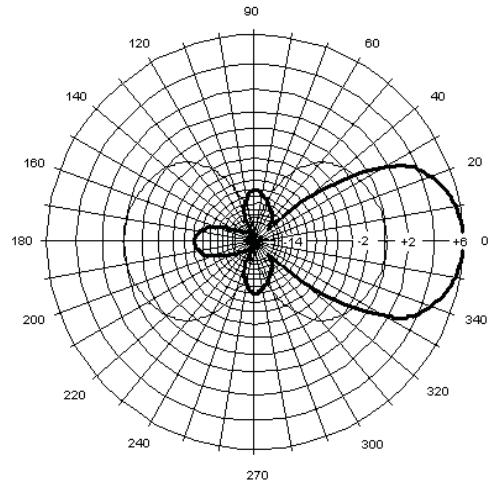
MYA8063 Vertical Pattern
