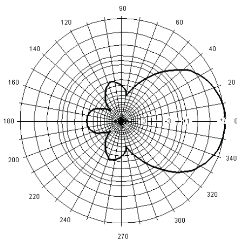
MYA1503 Horizontal Pattern
