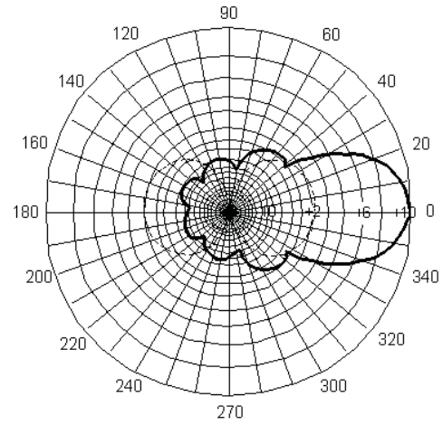
MYA9309 Vertical Pattern
