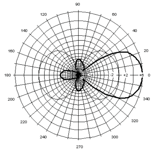
MYA9303 Vertical Pattern
