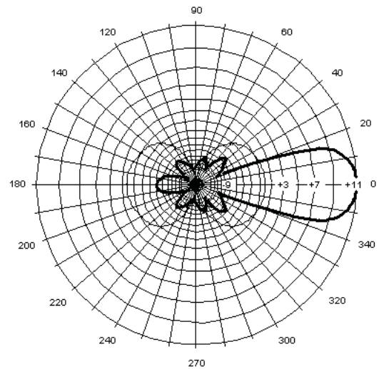
MYA80612 Vertical Pattern
