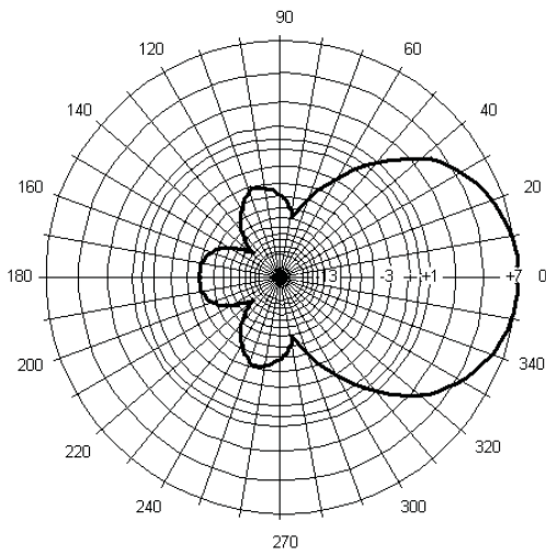
MYA723 Horizontal Pattern
