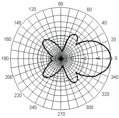
MYA9309 Horizontal Pattern
