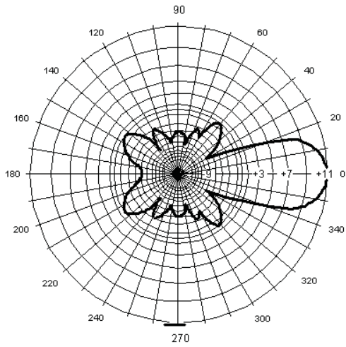
MYA93012 Horizontal Pattern
