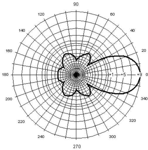
MYA8066 Horizontal Pattern
