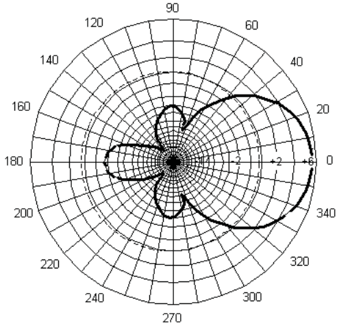
MYA8063 Horizontal Pattern
