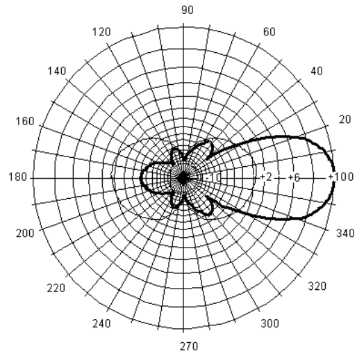
BMOY1506 Vertical Pattern
