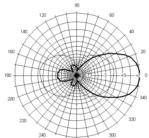
MYA1503 Vertical Pattern
