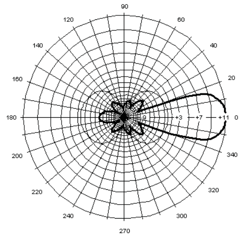
MYA93012 Vertical Pattern
