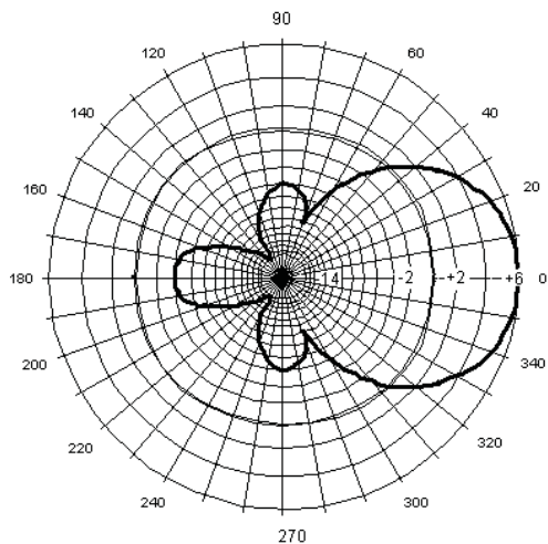
MYA9153 Horizontal Pattern
