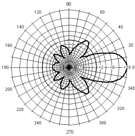
BMOY1506 Horizontal Pattern
