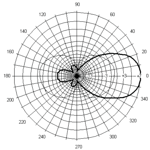
MYA723 Vertical Pattern
