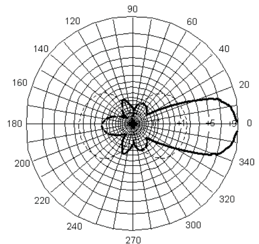
MYA9306 Vertical Pattern
