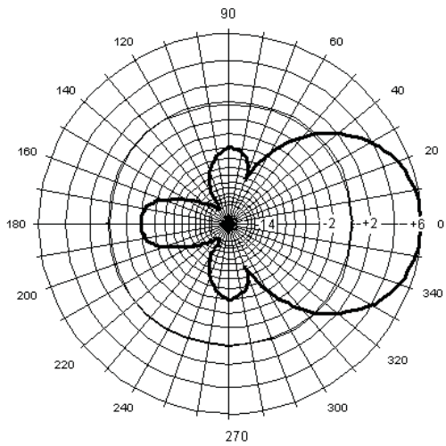
MYA9303 Horizontal Pattern
