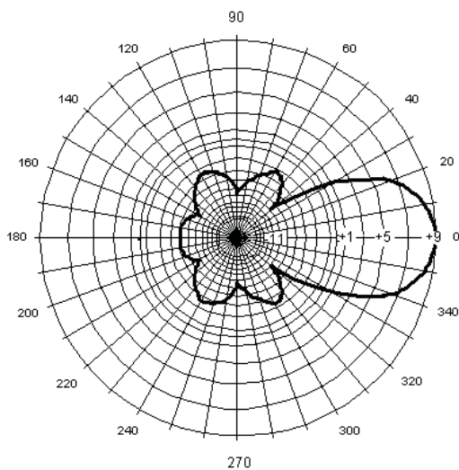
MYA9306 Horizontal Pattern
