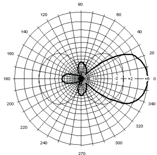
MYA9153 Vertical Pattern
