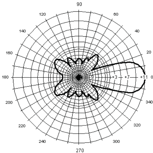
MYA80612 Horizontal Pattern
