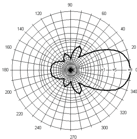
MYA1505 Horizontal Pattern
