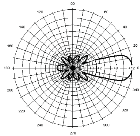
MYA45012 Vertical Pattern
