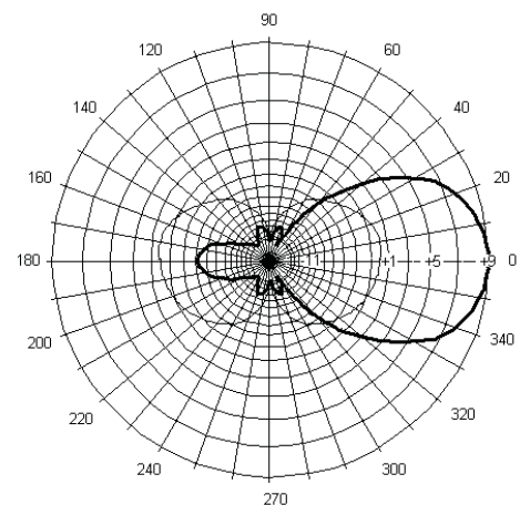
MYA1505 Vertical Pattern
