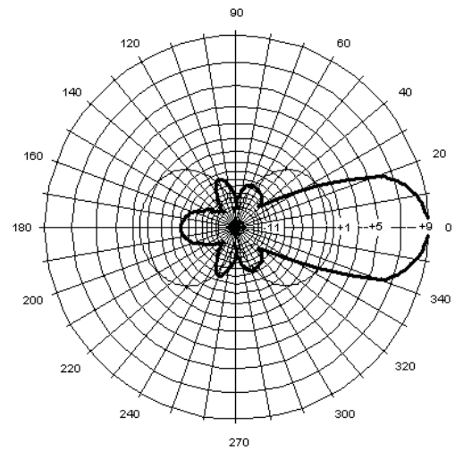
MYA8066 Vertical Pattern
